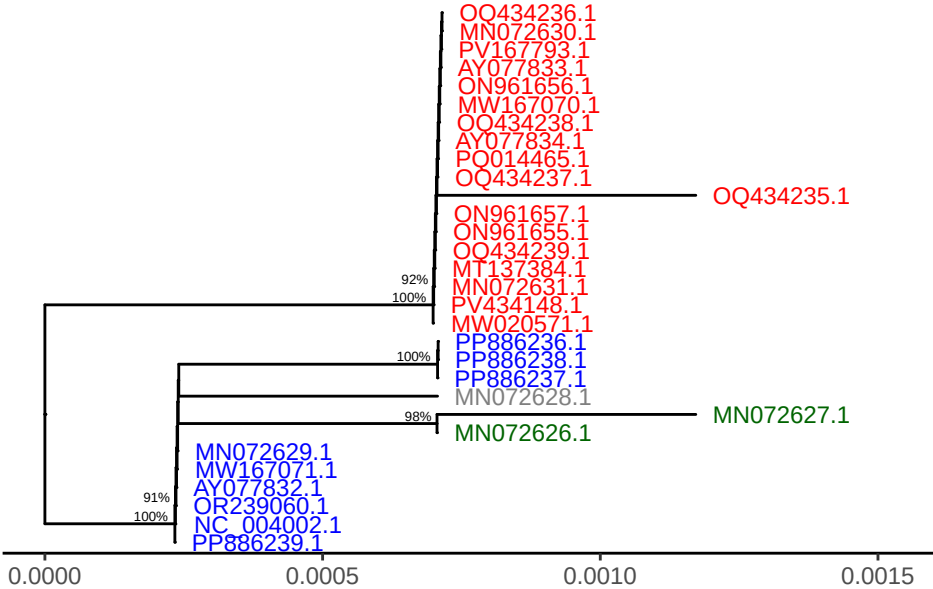
SPPV gene LSDV098
