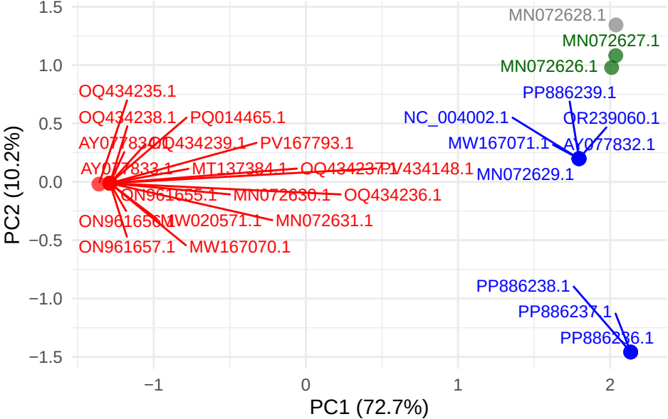
SPPV gene LSDV098
