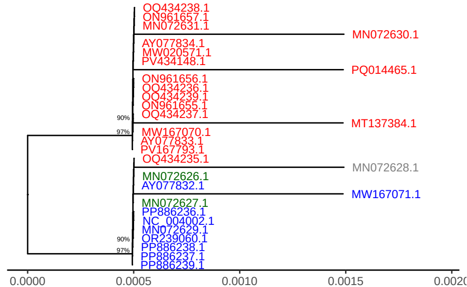
SPPV gene LSDV132
