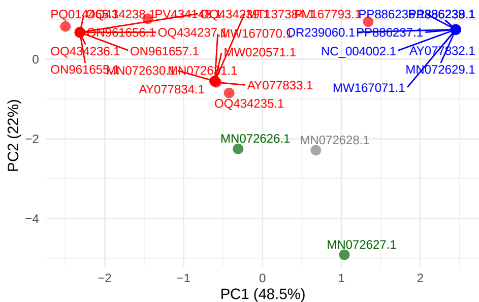
SPPV gene LSDV152
