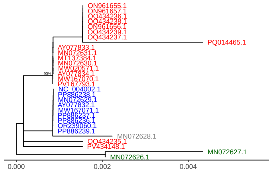
SPPV gene LSDV152
