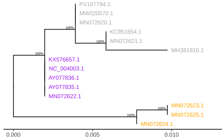
GTPV gene LSDV005
