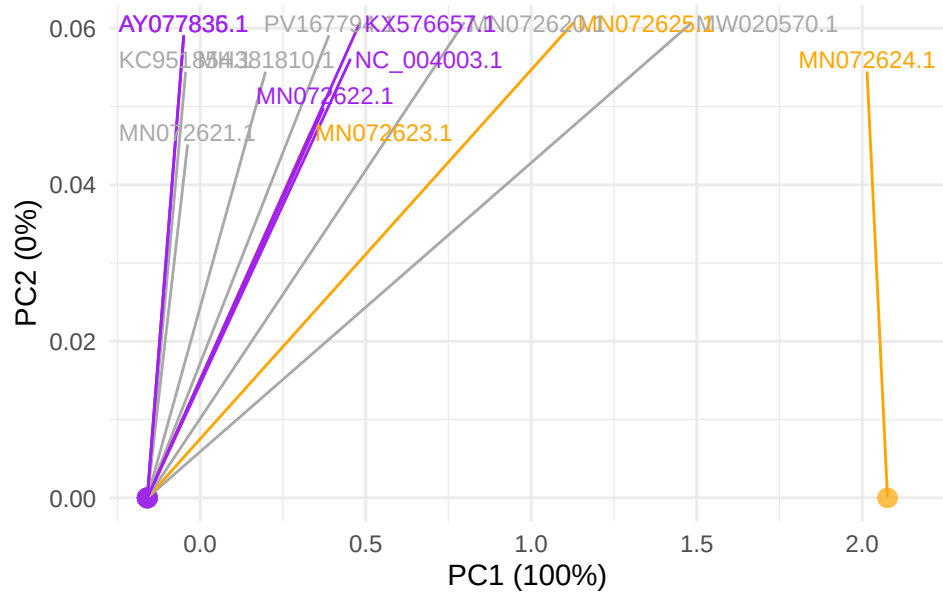
GTPV gene LSDV029
