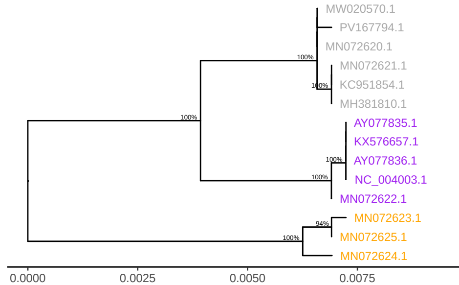
GTPV gene LSDV039
