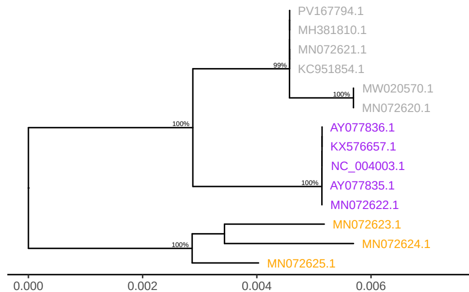
GTPV gene LSDV050
