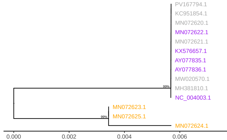
GTPV gene LSDV065
