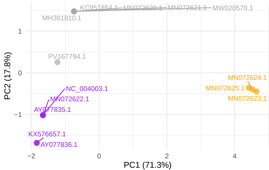
GTPV gene LSDV066
