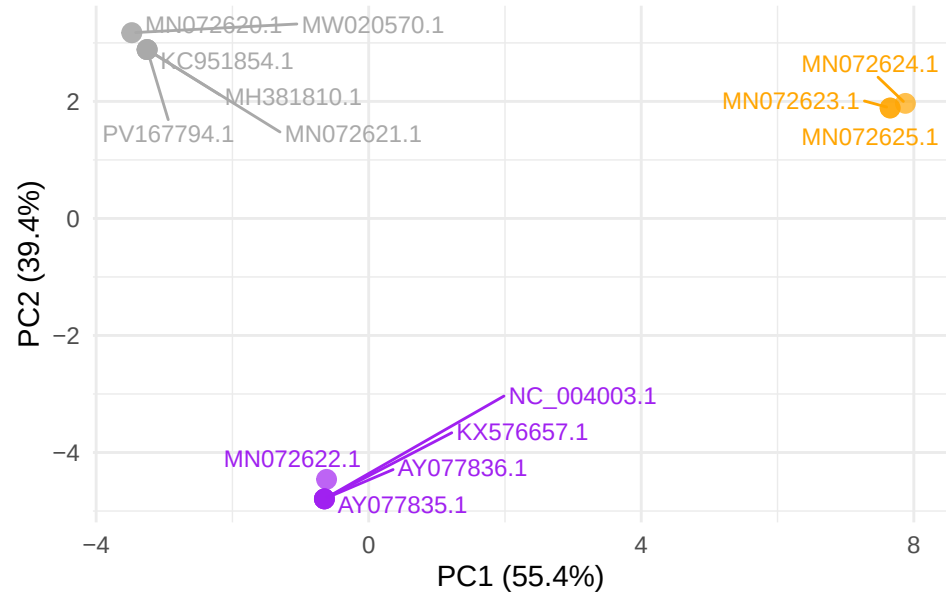
GTPV gene LSDV071
