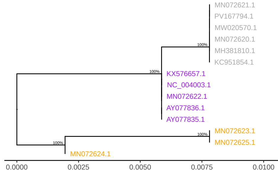
GTPV gene LSDV072
