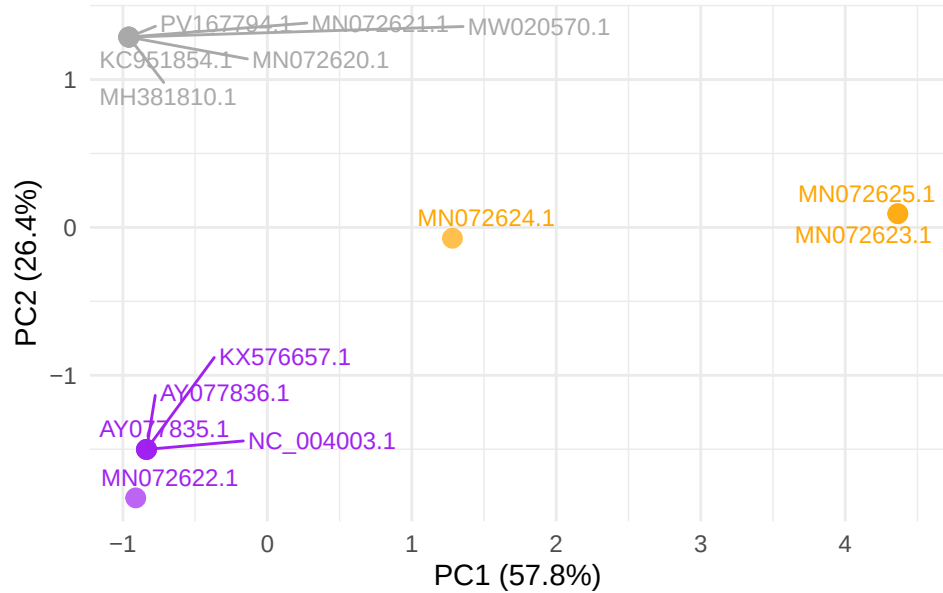
GTPV gene LSDV077
