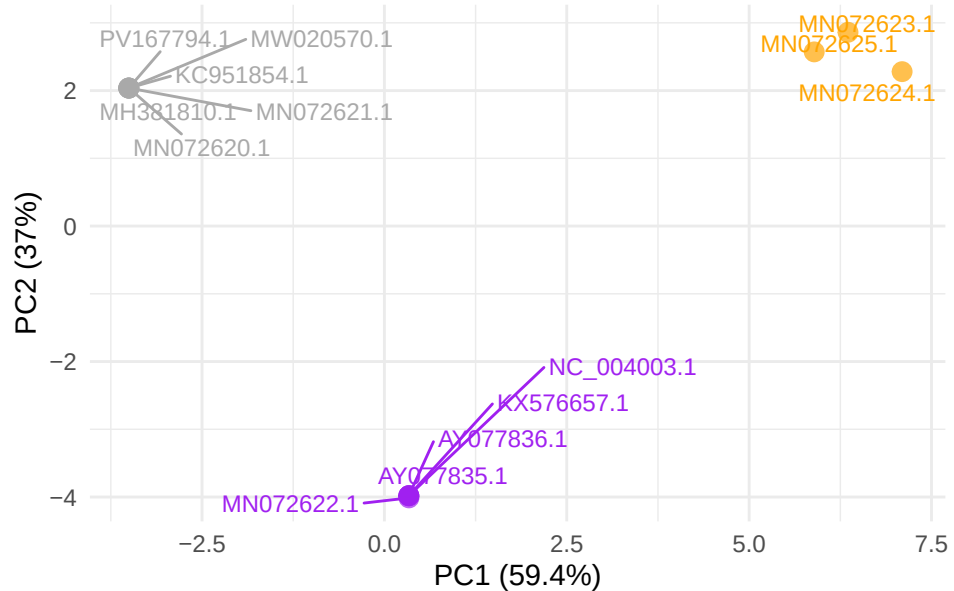
GTPV gene LSDV094
