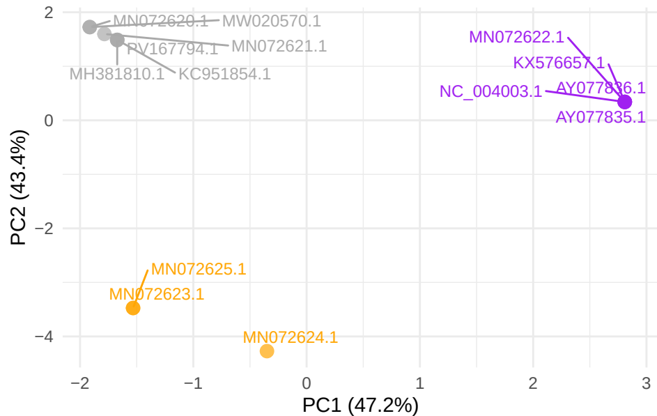
GTPV gene LSDV097
