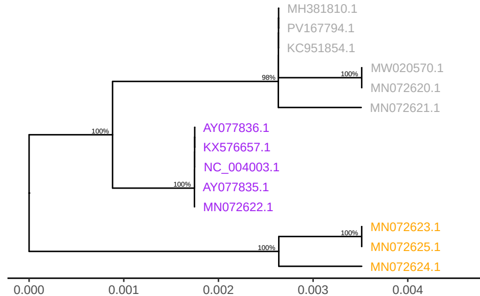
GTPV gene LSDV097
