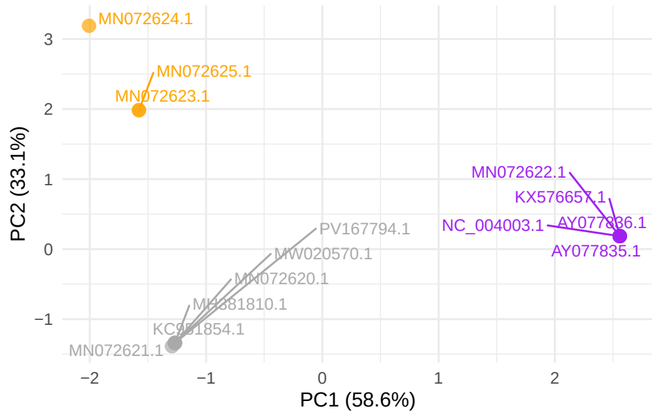
GTPV gene LSDV126
