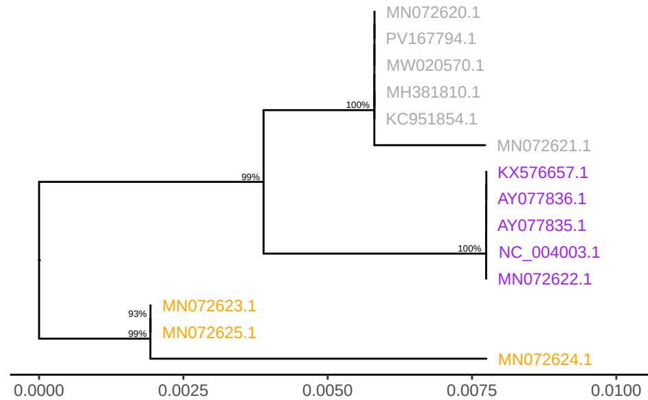
GTPV gene LSDV126
