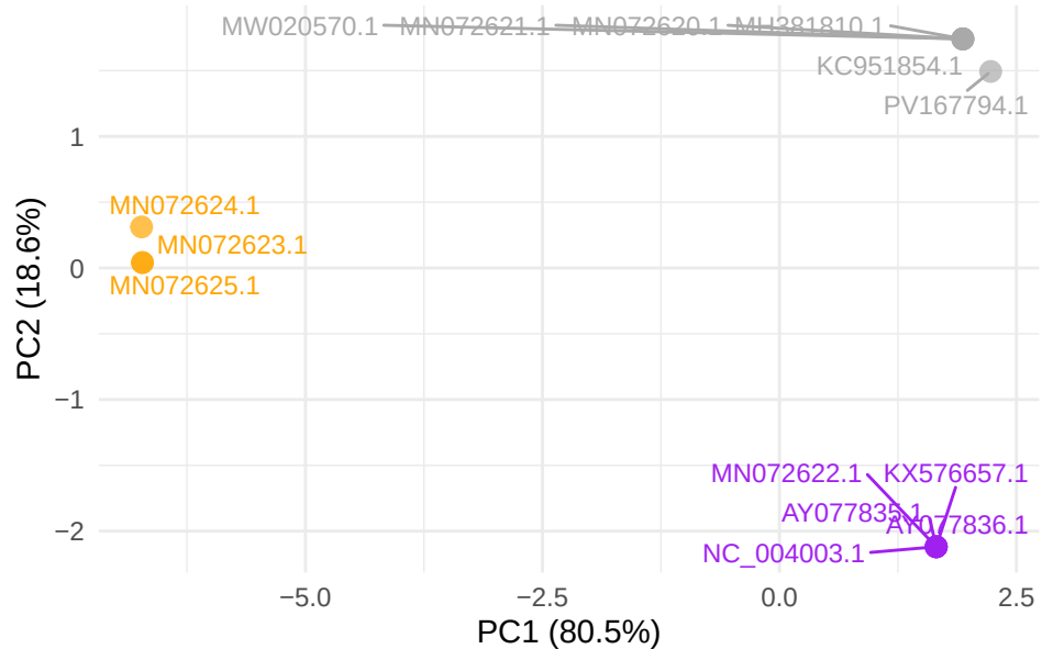
GTPV gene LSDV146
