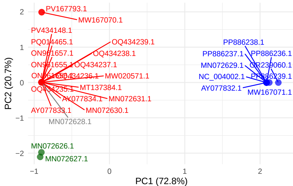
SPPV gene LSDV005
