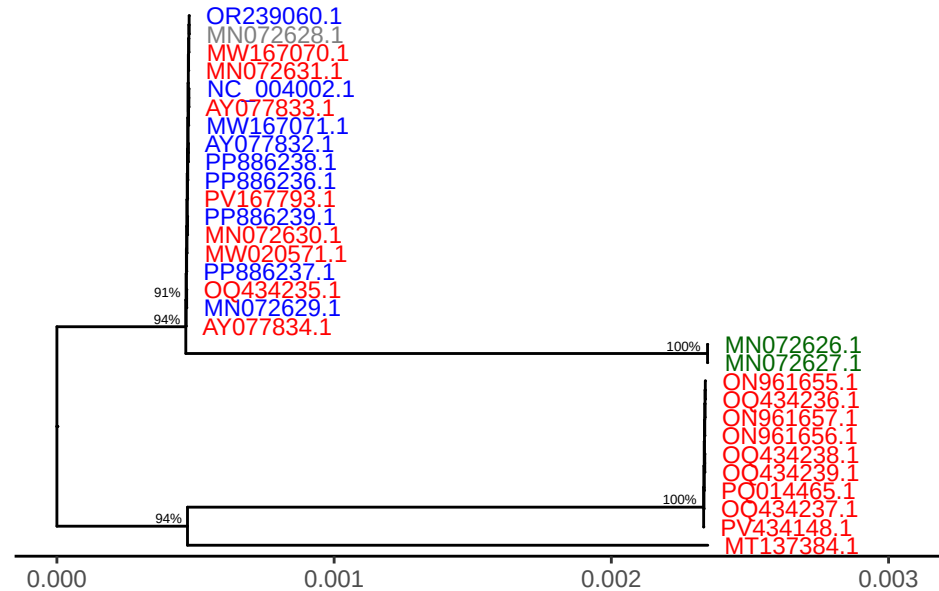
SPPV gene LSDV007
