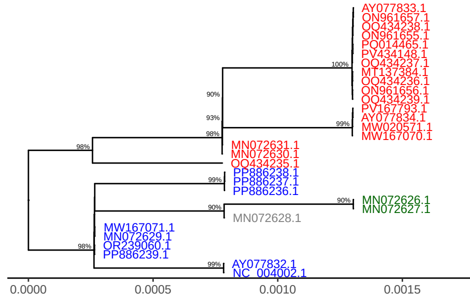
SPPV gene LSDV027
