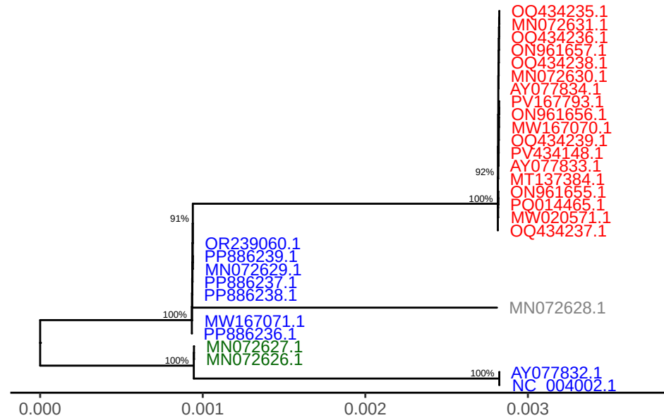
SPPV gene LSDV034
