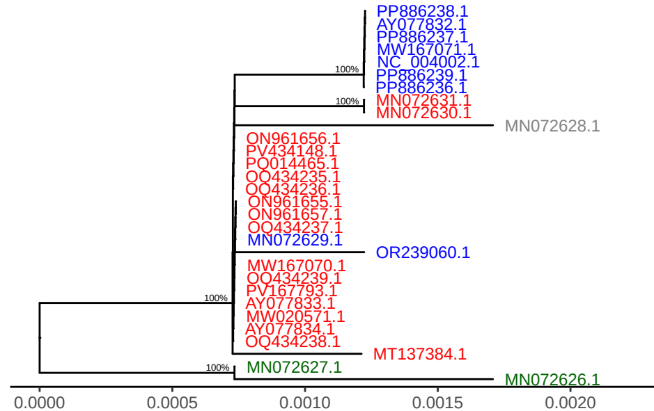
SPPV gene LSDV042
