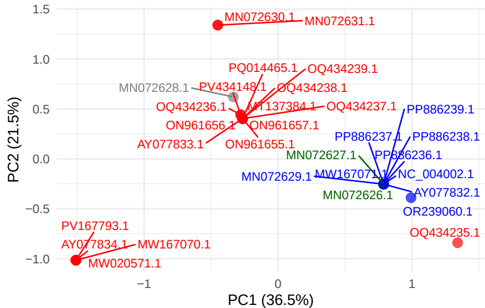
SPPV gene LSDV049
