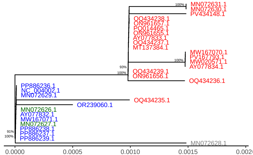
SPPV gene LSDV049
