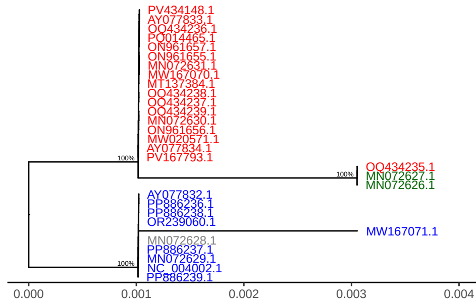
SPPV gene LSDV085
