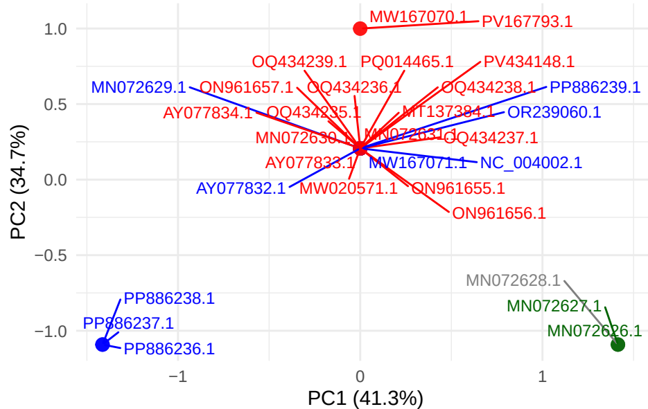
SPPV gene LSDV095
