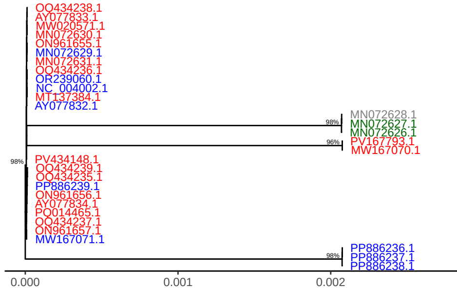
SPPV gene LSDV095
