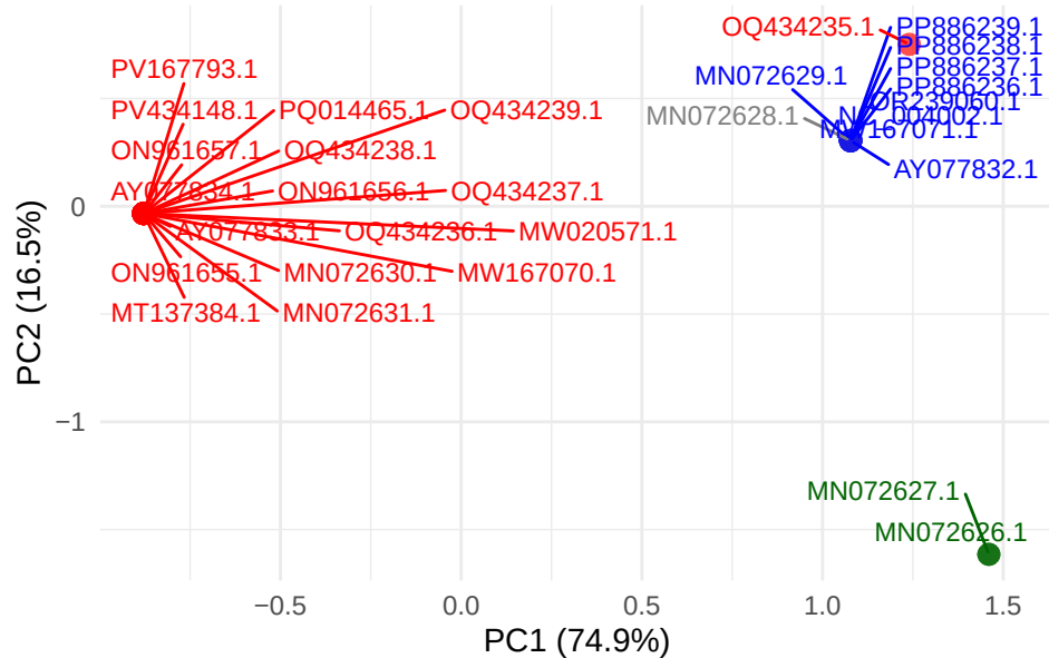
SPPV gene LSDV096
