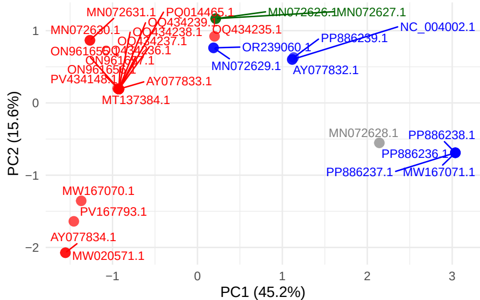
SPPV gene LSDV101
