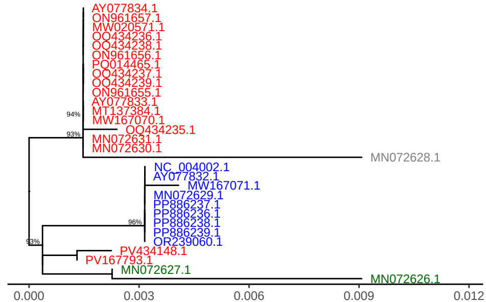
SPPV gene LSDV135
