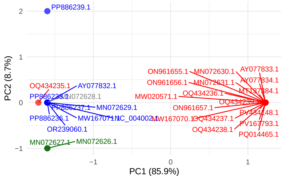
GTPV gene LSDV003
