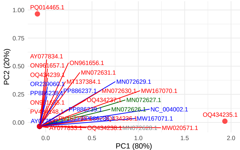
GTPV gene LSDV004
