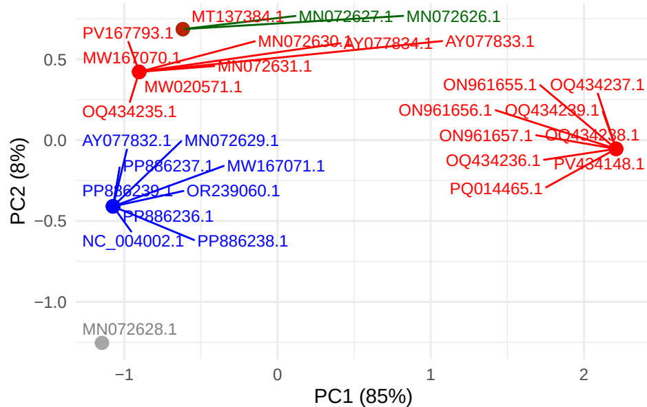
GTPV gene LSDV015
