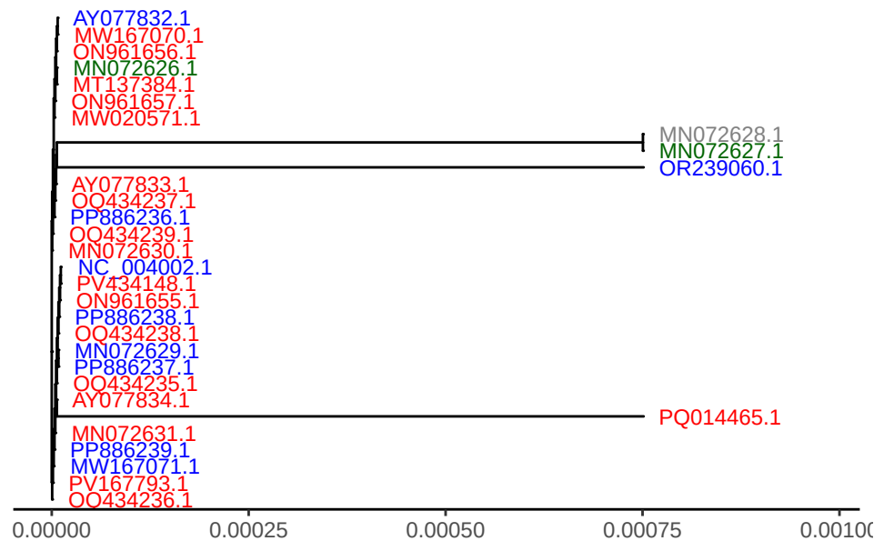
GTPV gene LSDV025
