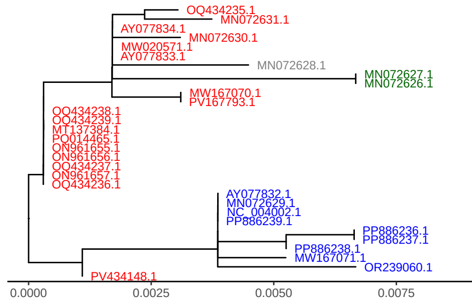
GTPV gene LSDV026
