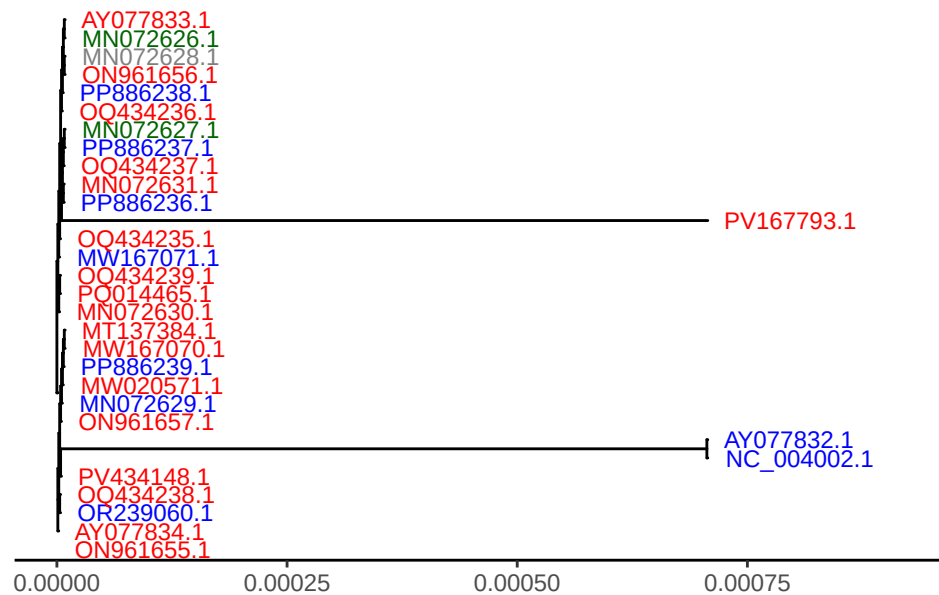
GTPV gene LSDV032
