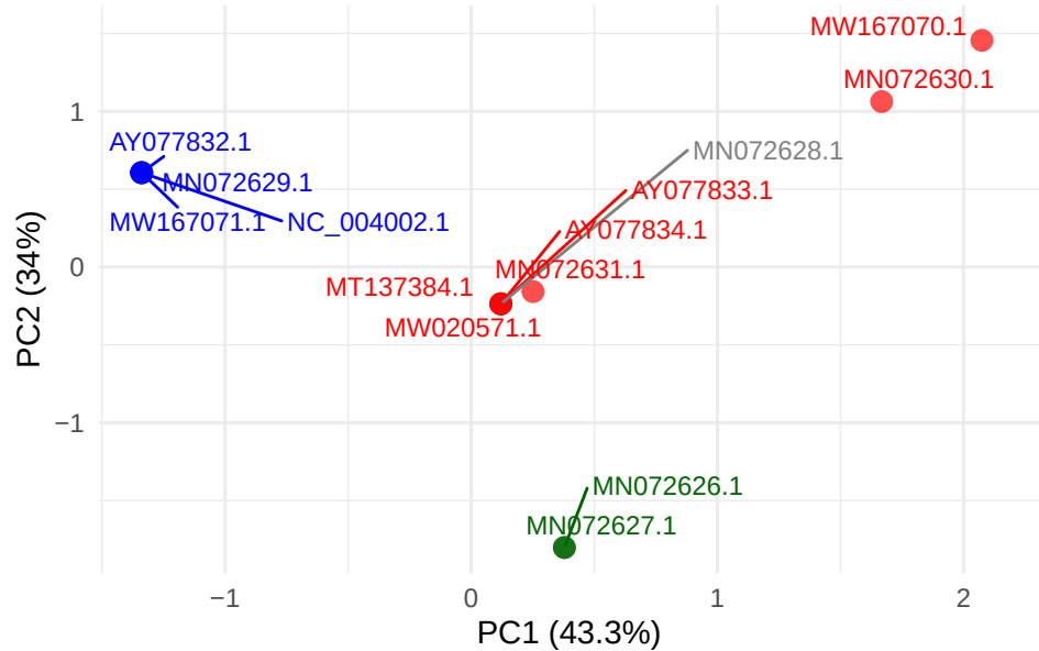
GTPV gene LSDV033
