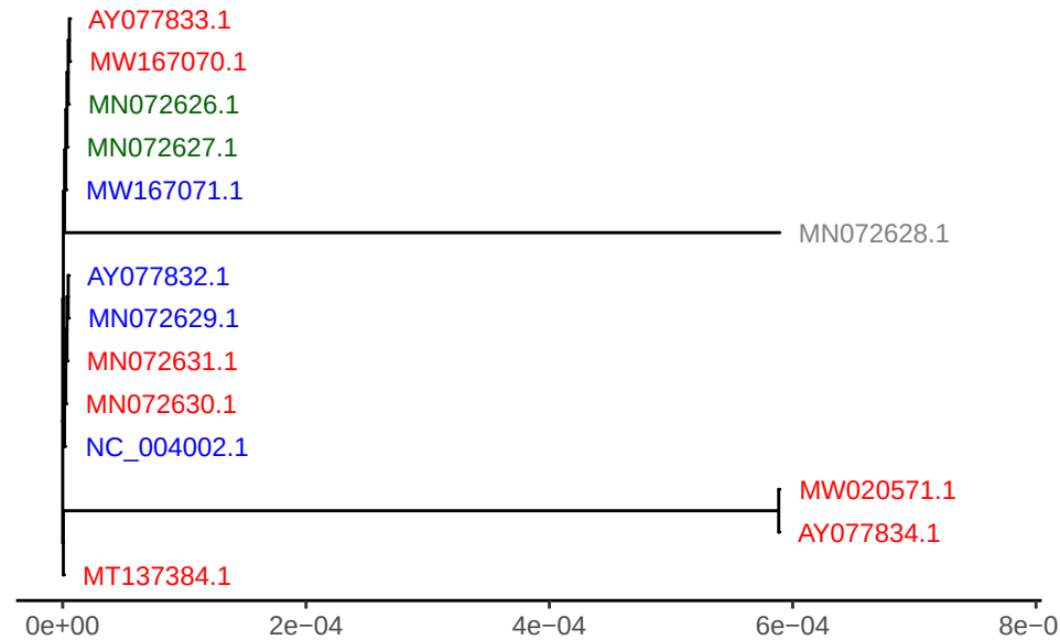
GTPV gene LSDV037
