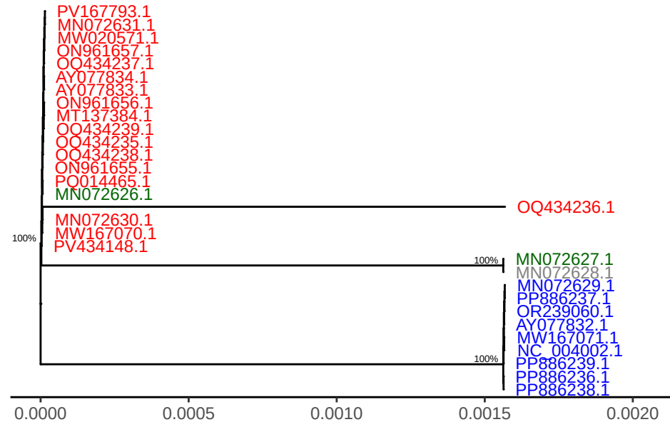
SPPV gene LSDV086
