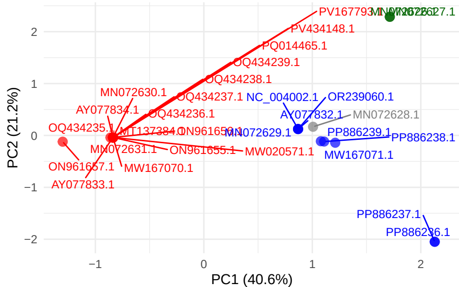
SPPV gene LSDV128
