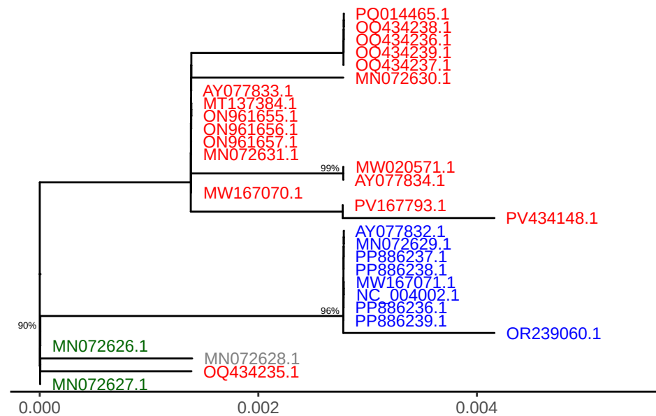
SPPV gene LSDV154
