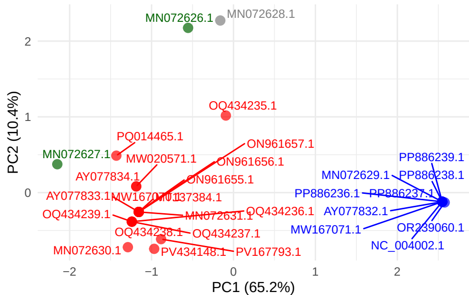
SPPV gene LSDV154
