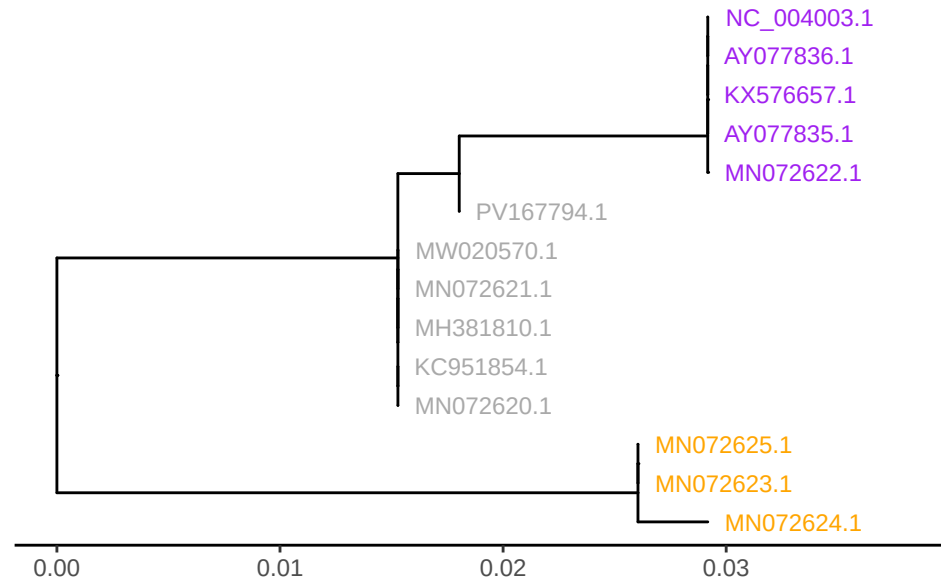
GTPV gene LSDV002
