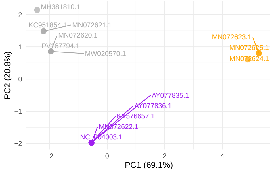
GTPV gene LSDV006
