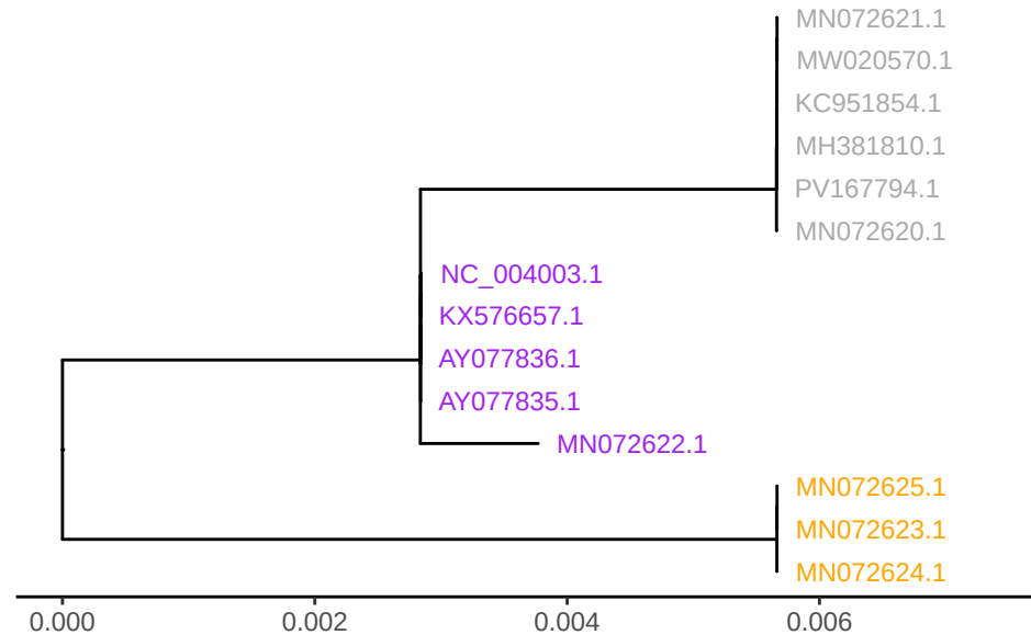
GTPV gene LSDV007
