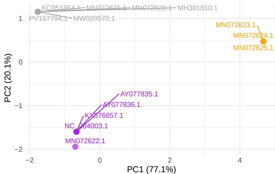
GTPV gene LSDV007
