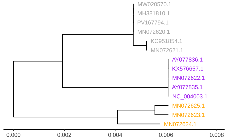
GTPV gene LSDV027
