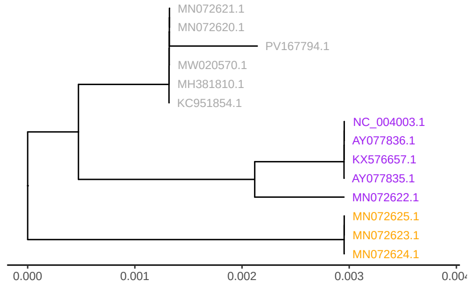
GTPV gene LSDV035
