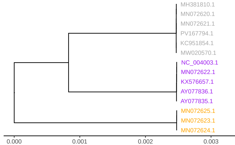
GTPV gene LSDV036
