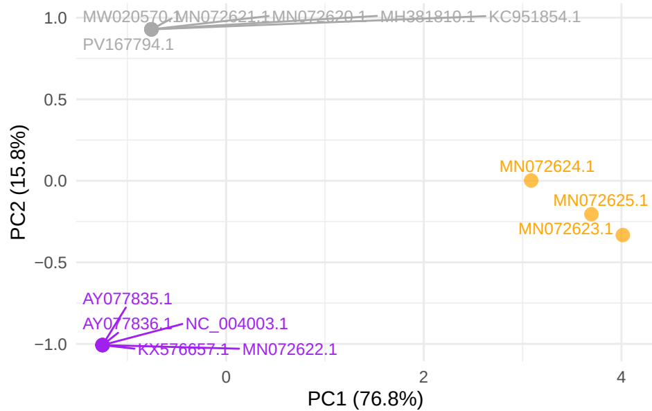
GTPV gene LSDV041
