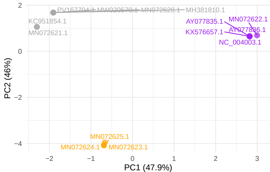
GTPV gene LSDV048
