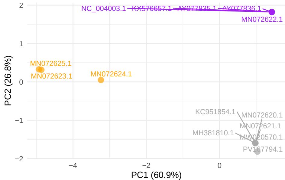
GTPV gene LSDV054
