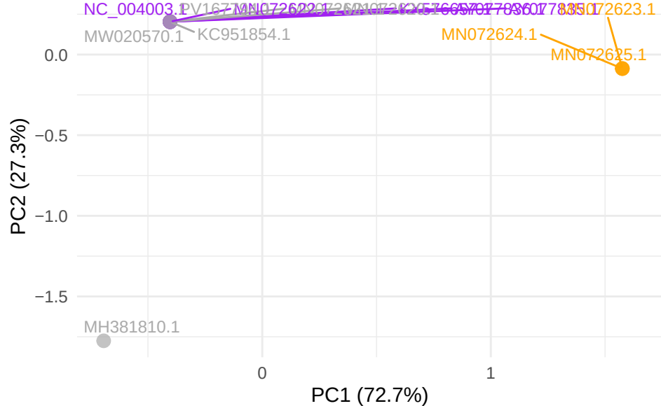
GTPV gene LSDV055
