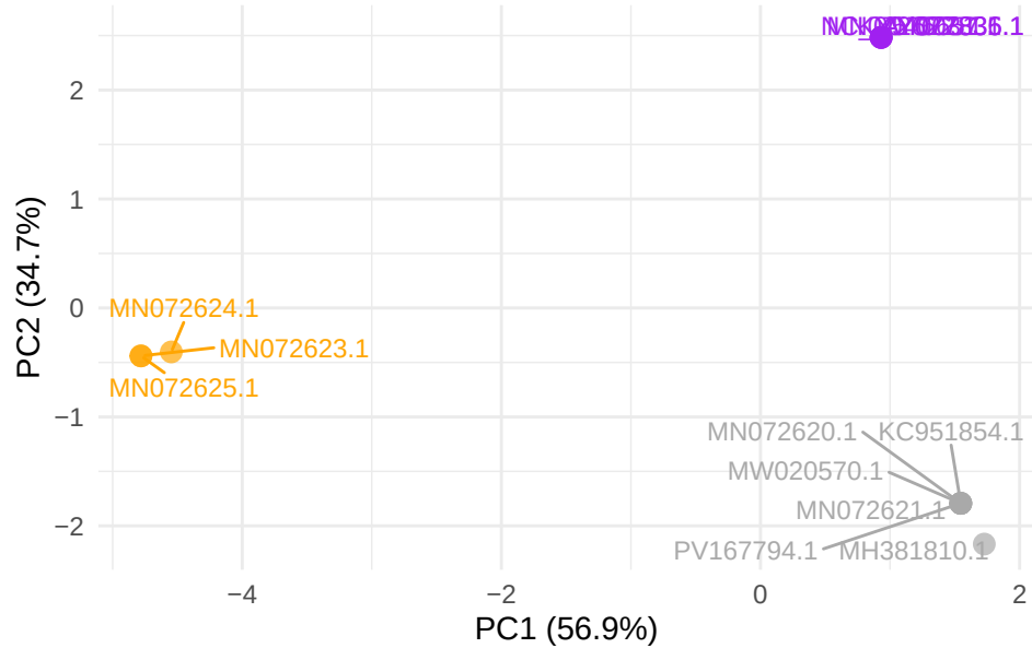
GTPV gene LSDV059
