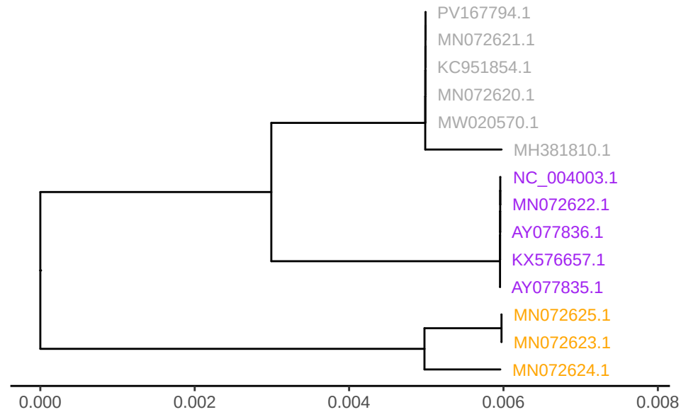
GTPV gene LSDV059
