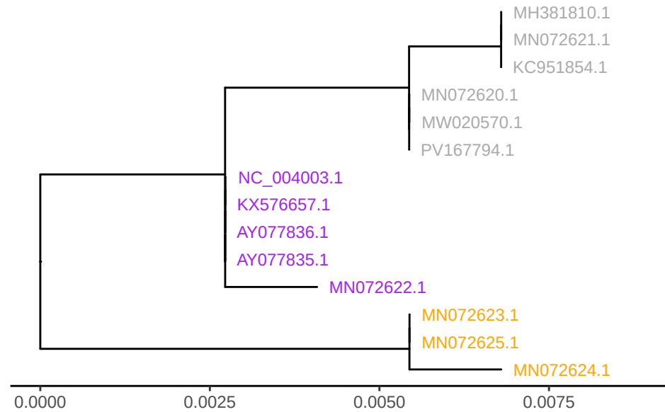
GTPV gene LSDV060
